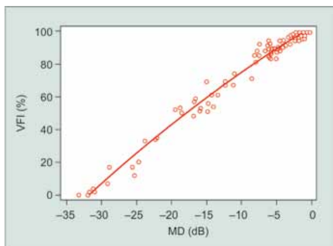
Graph 1: Correlation between VFI and MD (MD: Mean deviation; VFI: Visual field index)
