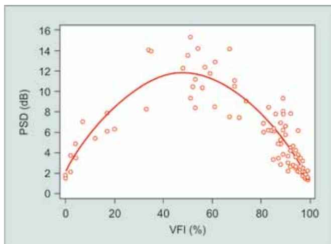
Graph 3: Nonlinear correlation between VFI and PSD (PSD: Pattern standard deviation; VFI: Visual field index)
