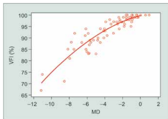
Graph 2: Nonlinear correlation between MD and VFI considering only the eyes with early and moderate functional damage (MD: Mean deviation; VFI: Visual field index)
