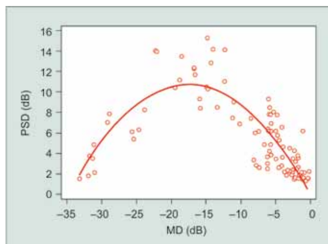
Graph 4: Nonlinear correlation between MD and PSD (PSD: Pattern standard deviation; MD: Mean deviation)
